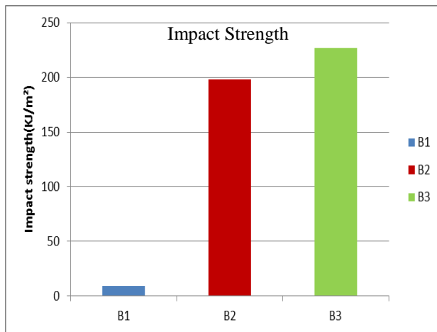
Figure 6: Hybrid polymer blend matrix composites' impact strength. B1, B2, and B3 refer to the samples.
