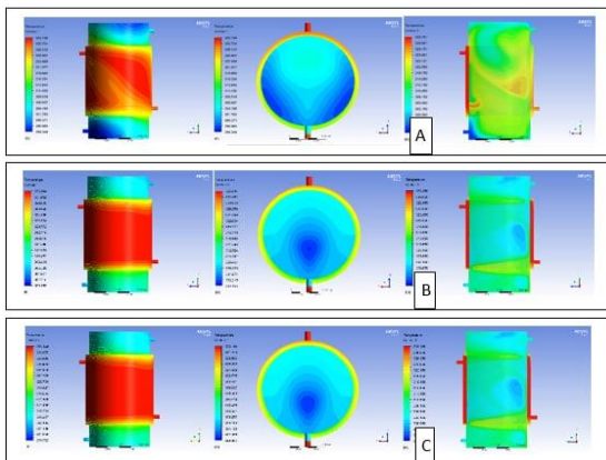
Figure 4. Temperatures contours of the tank (right and middle) and mantle (left) at mantle gap of 10 mm and mantle length of 300 mm for mass flow rate: (A) \dot{m} = 0.0077 kg/s, (B) \dot{m} = 0.015 kg/s, (C) \dot{m} = 0.02 kg/s, at 1800s.
