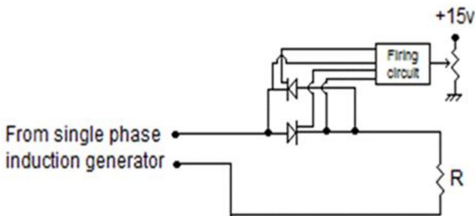
Fig .(13) Schematic diagram of nonlinear load (thyristorac chopper in series with resistive load)fed from single phase induction generator.
