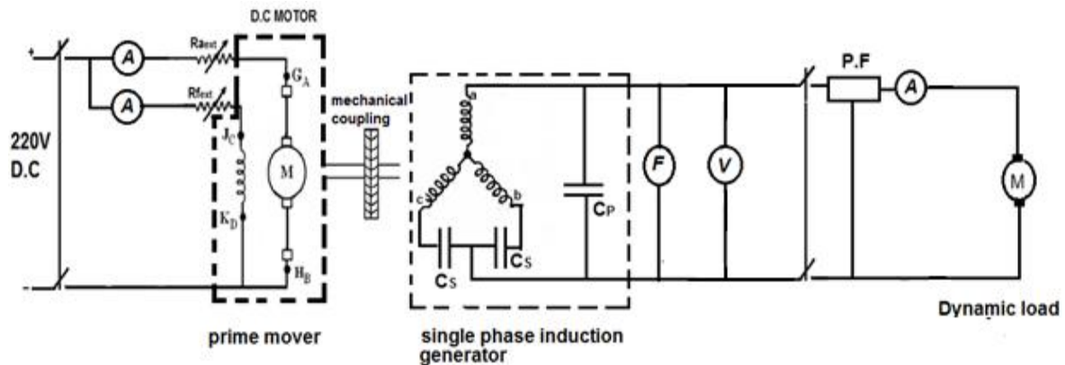
Fig .(10) Schematic diagram of single feeding single phase induction generator phase induction motor.
