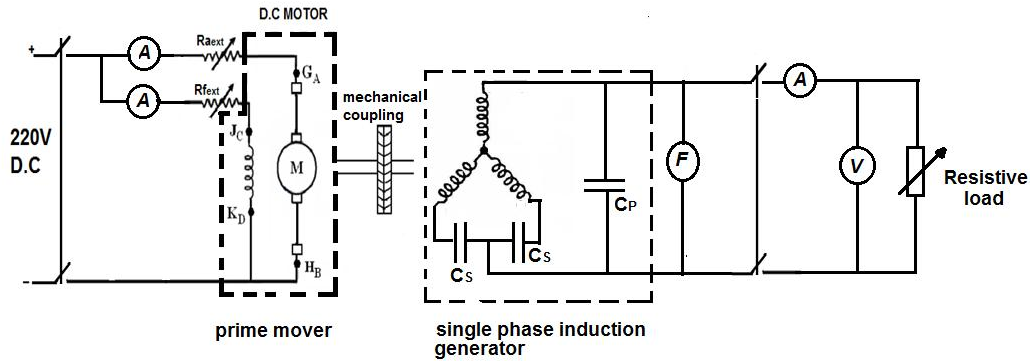
Fig .(3) Schematic diagram of the experimental setup with resistive load.
