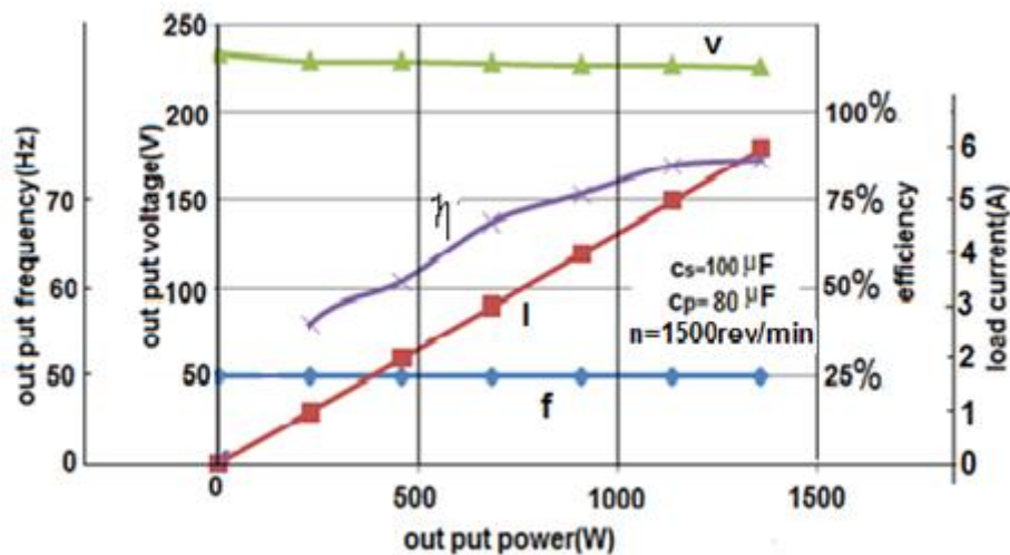
Fig .(4) Load characteristics for resistive load with C_s = 100\mu\text{F} and C_p = 80\mu\text{F} .
