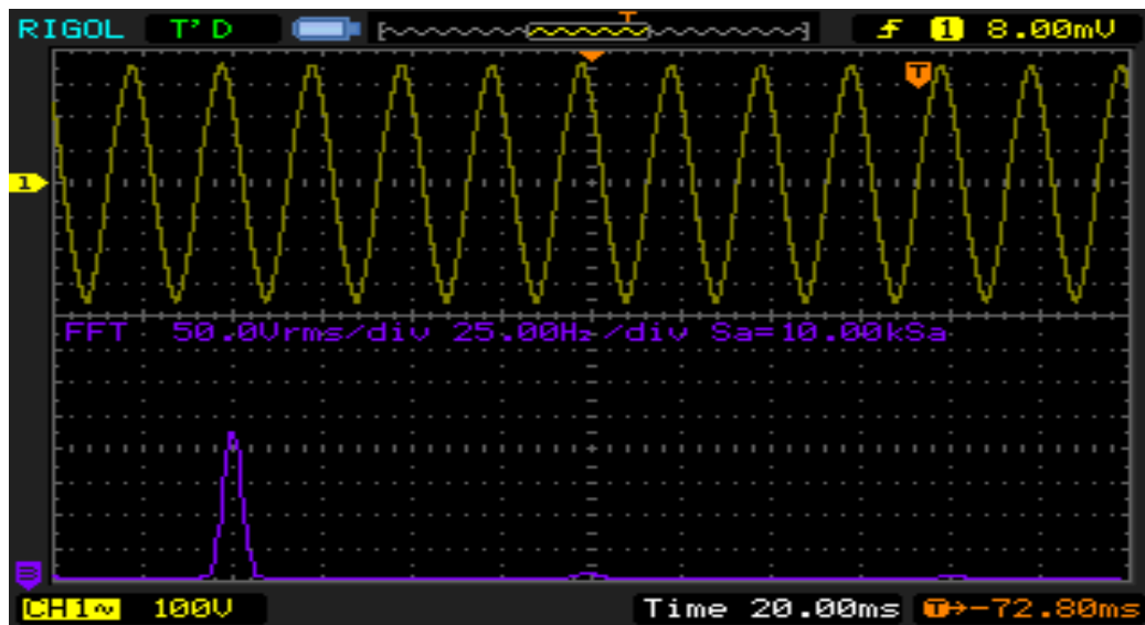
Fig .(11) Waveform and harmonics spectrum of output voltage of single phase generator feeding permanent capacitor single phase induction motor
