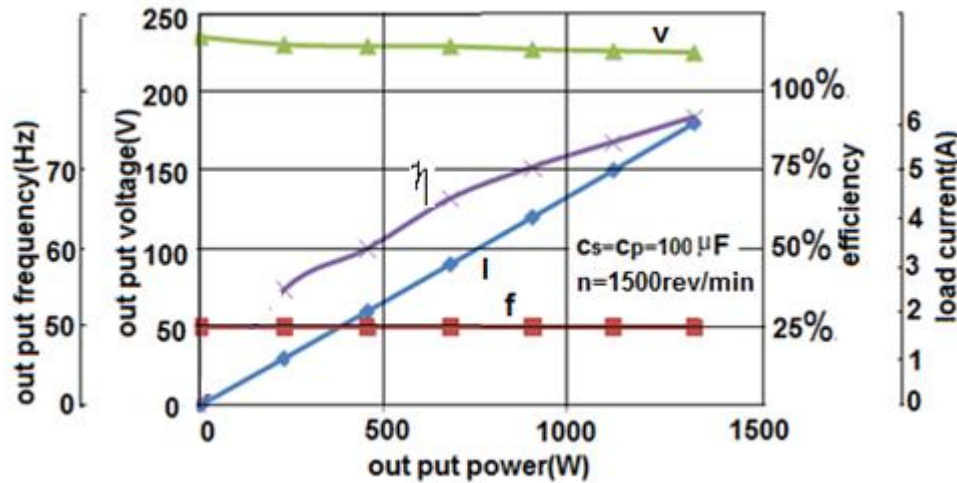
Fig .(5) Load characteristics for resistive load with C_s=C_p=100\mu\text{F} .
