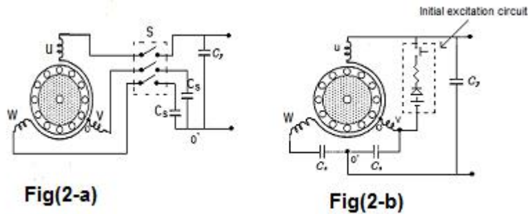
Fig .(2) Circuit diagram showing the methods of voltage build-up .
