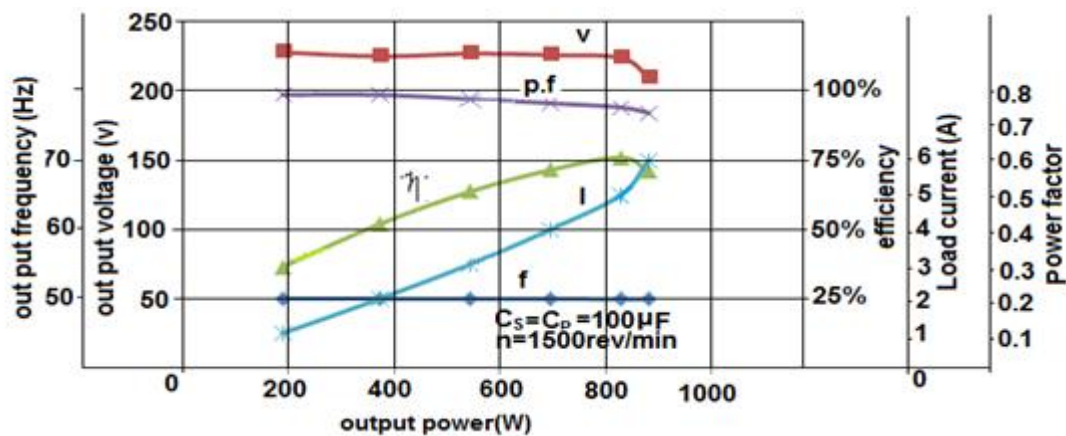
Fig .(7) Load characteristics for inductive load with C_s=C_p=100\mu\text{F}
