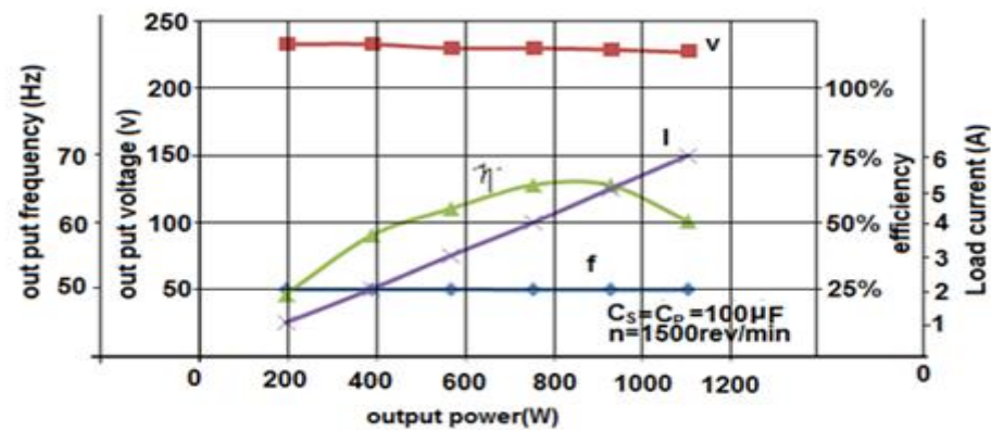
Fig .(8) Load characteristics for inductive load with C_s=C_p=100\mu F and constant power factor of 0.8
