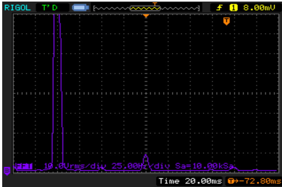
Fig .(12) Harmonics spectrum of output voltage for single phase induction generator feeding capacitor-start single phase induction motor. 3-2-4 Results for non-linear load using thyristor AC chopper
