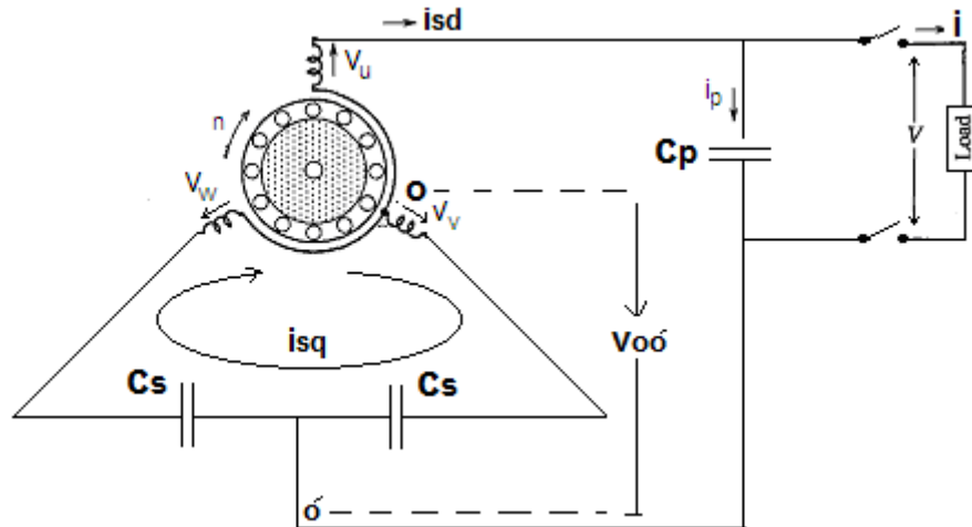
Fig.(1) Schematic diagram of the capacitor self-excited single-phase induction generator [5].
