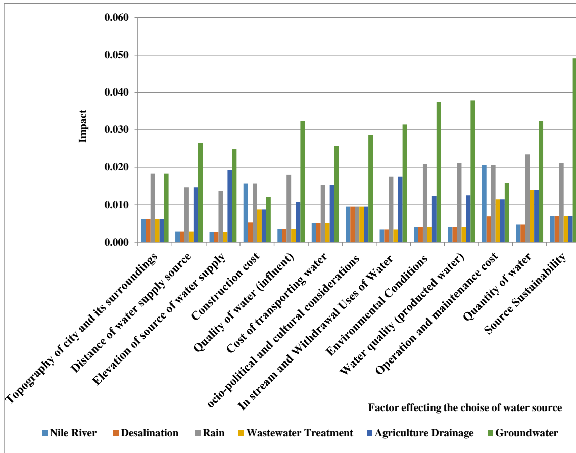
Figure 6. Impact of each resource concerning each factor for the Western Desert Zone
