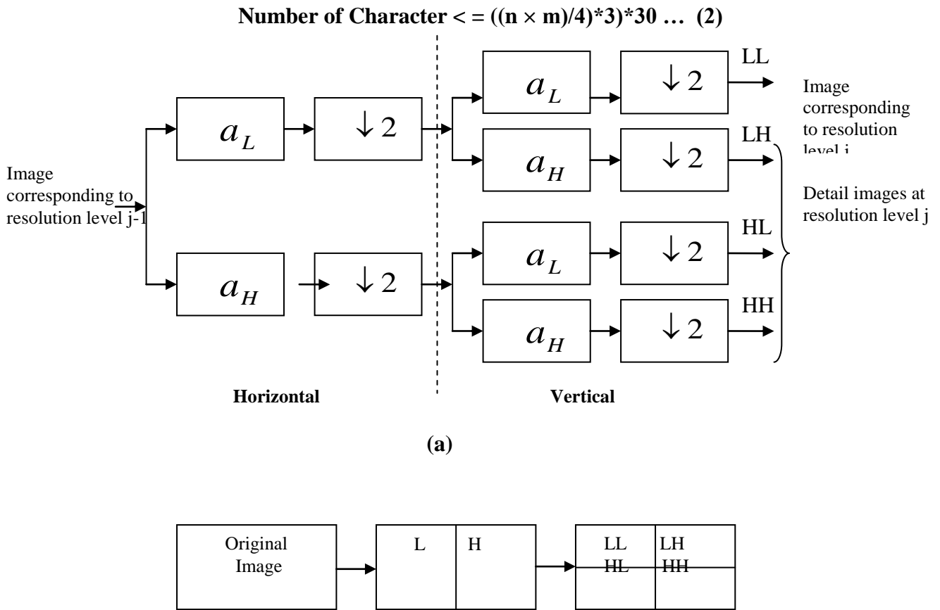
Figure 3: (a) One Filter Stage in 2-D DWT, (b) Pyramidal Structure of a Wavelet
