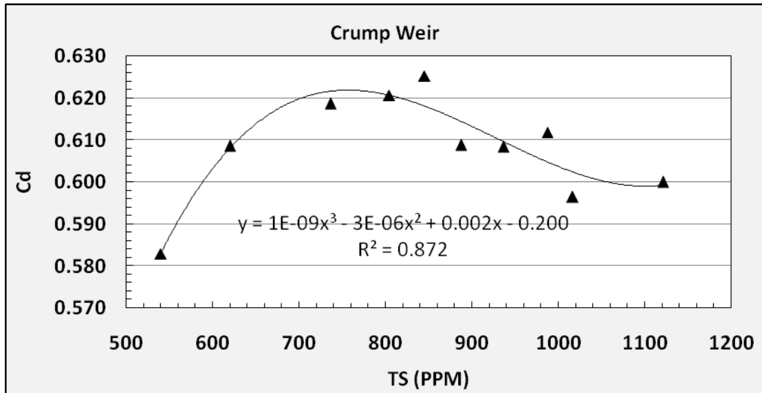
Fig.(6-b): Effect of the total solid TS on the values of discharge coefficient Cd in the Crump weir.
