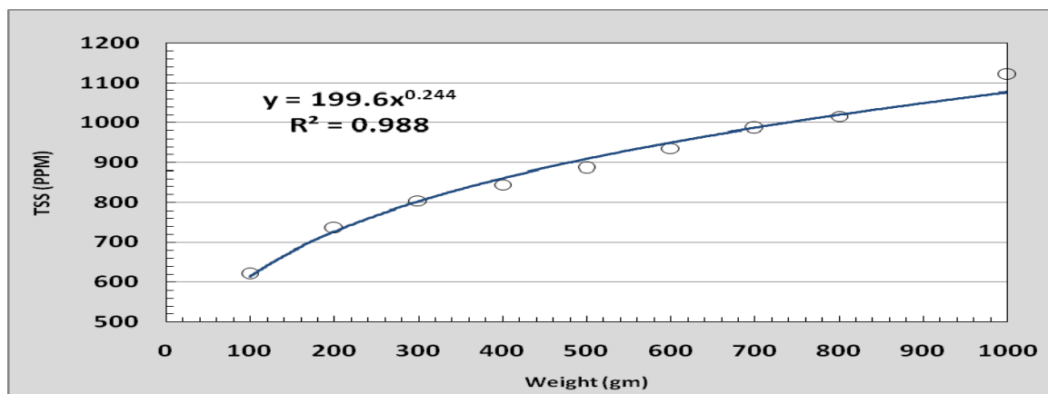
Figure(5): Weight of dried soil and TS Relationship.
