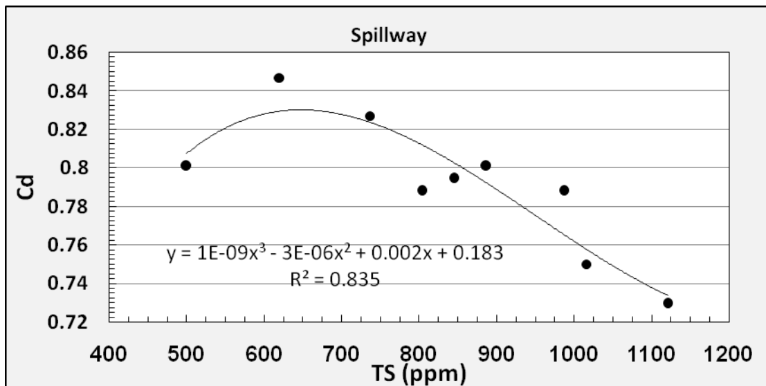
Fig.(6-c): Effect of the total solid TS on the values of discharge coefficient Cd in the spillway.
