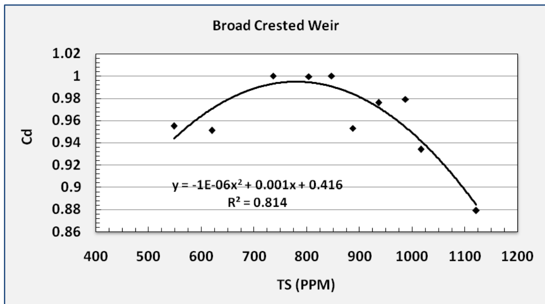
Fig.(6-a): Effect of the total solid TS on the values of discharge coefficient C_d in the Broad crested weir.
